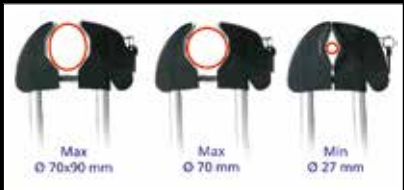
IN NERO, DISPOSITIVO BREVETTATO PER TUBI DI PICCOLO DIAMETRO IN BLACK, CLOSE-UP PATENTED OF CLAMP JAW REDUCER CLOSE UP OF CLAMP
